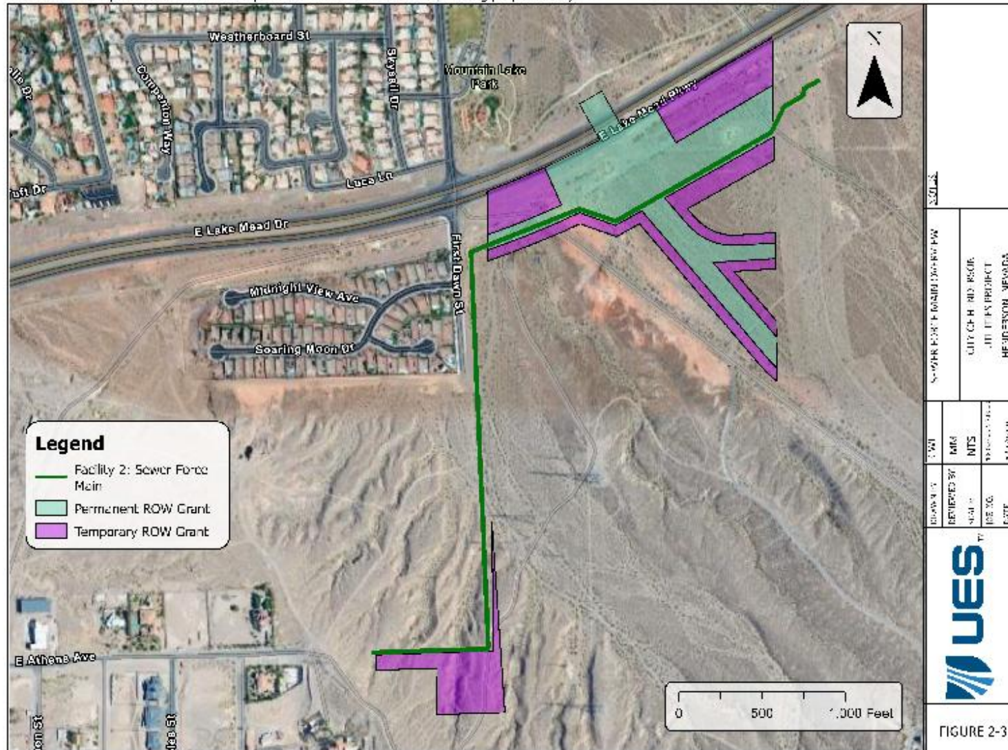
Figure 2-3: Sewer Force Main Overview
